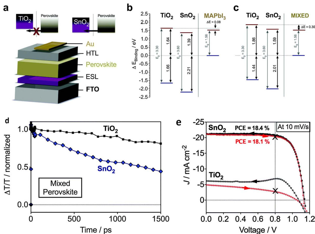
Fig. 21 (a–c). Diagram of energy level plans and electron inoculation properties of SnO 2 - and TiO 2 -based planar PSCs, (d) transient absorption findings, (e) current–voltage ( J-V ) curves of TiO 2 - and SnO 2 -based planar mixed halide-mixed cation PSCs (reproduced with permission from ref. 184. Copyright 2015 RSC).
