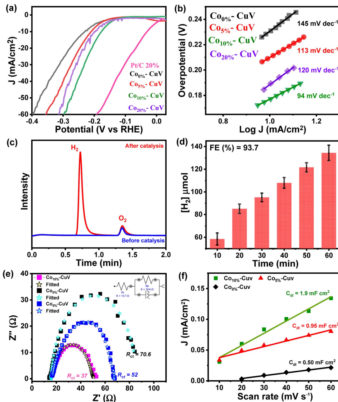
Fig. 3 (a) Comparative linear sweep voltammograms (LSVs) and (b) Tafel plots for the HER on modified GCEs comprising pure CuV ( \text{Co}_{0\%} -CuV) (black trace), Co-doped copper vanadates ( \text{Co}_{5\%} -CuV) (red trace), \text{Co}_{10\%} -CuV (green trace), and \text{Co}_{20\%} -CuV (violet trace) in 1.0 M KOH. A standard three electrode set up consisting of a copper vanadate immobilized glassy carbon disc (5 mm diameter) working electrode, Pt wire counter electrode, and Ag/AgCl (3.0 M KCl) reference electrode was used here at 298 K under 1 atm \text{N}_2 . A scan rate of 5 \text{ mV s}^{-1} was maintained for all the experiments. (c) Gas chromatography (GC) analysis during chronoamperometry of \text{Co}_{10\%} -CuV for the HER [before electrocatalysis (blue trace) and after electrocatalysis (red trace)], and (d) the serial evolution of \text{H}_2 during the bulk electrocatalysis by \text{Co}_{10\%} -CuV during the bulk electrolysis experiment. (e) The comparative EIS spectra of Co(II) doped modified electrodes were measured in 1.0 M KOH solution at an open circuit potential and with input frequencies ranging from 100 kHz to 0.01 Hz. (f) Capacitive currents for doped and undoped copper vanadate at 0.05 V as a function of scan rate.
