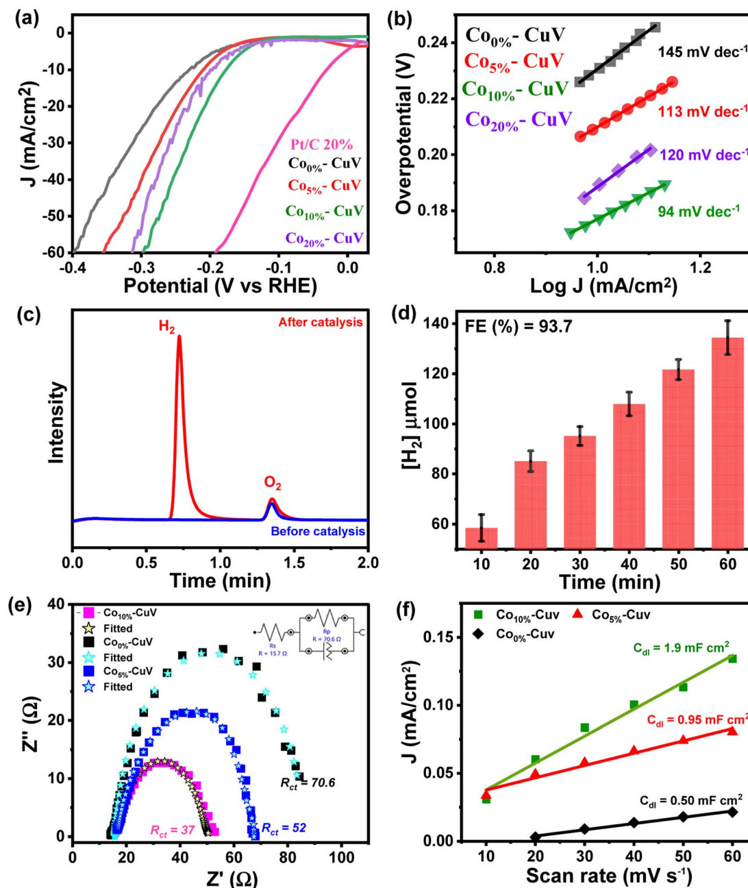
Fig. 3 (a) Comparative linear sweep voltammograms (LSVs) and (b) Tafel plots for the HER on modified GCEs comprising pure CuV ( \text{Co}_0\text{-CuV} ) (black trace), Co-doped copper vanadates ( \text{Co}_5\text{-CuV} ) (red trace), \text{Co}_{10}\text{-CuV} (green trace), and \text{Co}_{20}\text{-CuV} (violet trace) in 1.0 M KOH. A standard three electrode set up consisting of a copper vanadate immobilized glassy carbon disc (5 mm diameter) working electrode, Pt wire counter electrode, and Ag/AgCl (3.0 M KCl) reference electrode was used here at 298 K under 1 atm \text{N}_2 . A scan rate of 5 \text{ mV s}^{-1} was maintained for all the experiments. (c) Gas chromatography (GC) analysis during chronoamperometry of \text{Co}_{10}\text{-CuV} for the HER [before electrocatalysis (blue trace) and after electrocatalysis (red trace)], and (d) the serial evolution of \text{H}_2 during the bulk electrocatalysis by \text{Co}_{10}\text{-CuV} during the bulk electrolysis experiment. (e) The comparative EIS spectra of Co(II) doped modified electrodes were measured in 1.0 M KOH solution at an open circuit potential and with input frequencies ranging from 100 kHz to 0.01 Hz. (f) Capacitive currents for doped and undoped copper vanadate at 0.05 V as a function of scan rate.
