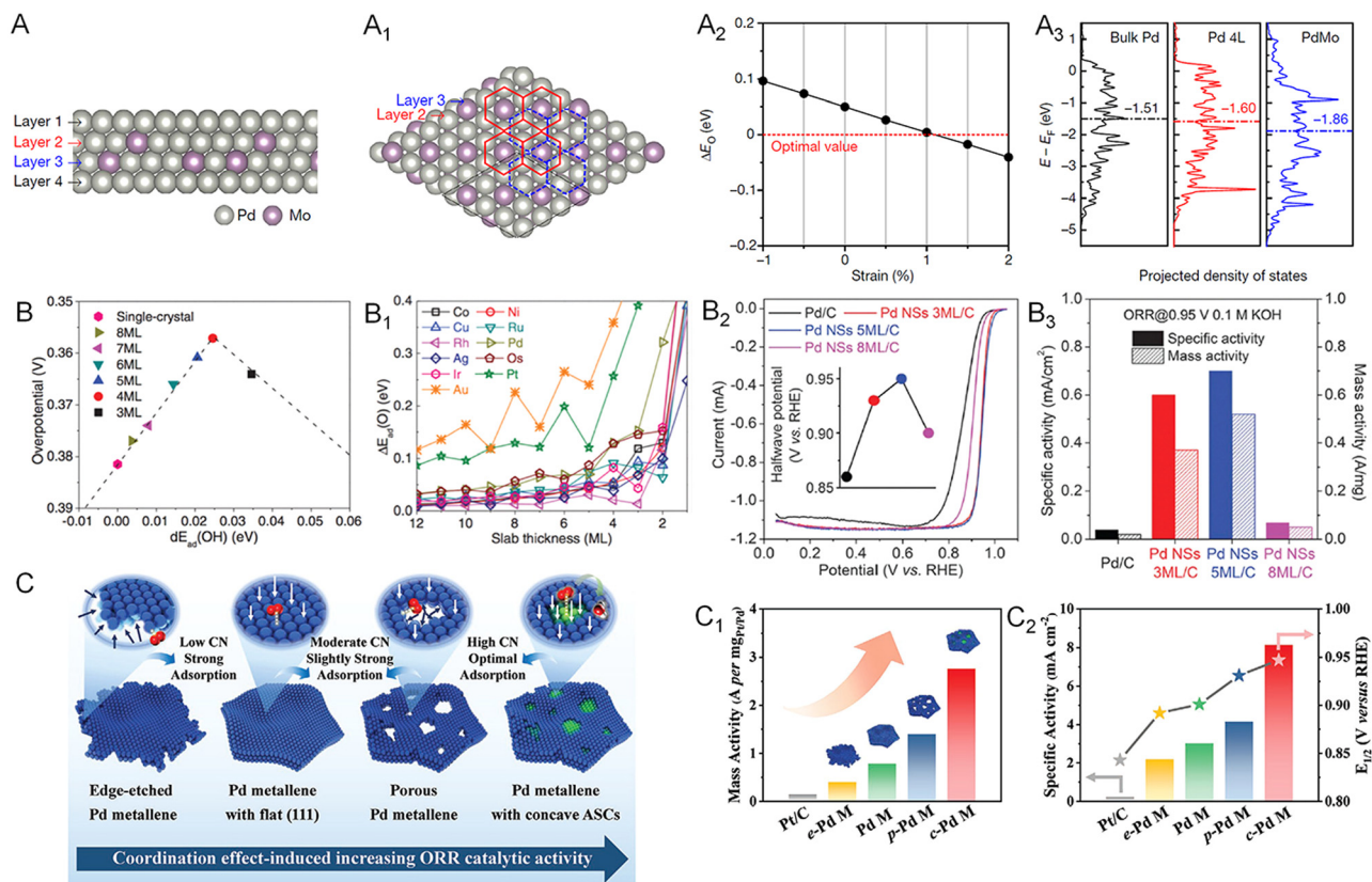
Fig. 10 Utilization of metallenes in the ORR. (A) Side and (A 1 ) top view of the atomic model of the four-layer PdMo bimetalene. (A 2 ) \Delta E_{O_2} of PdMo bimetalene as a function of compressive (negative) and tensile (positive) strains. (A 3 ) The projected electronic density of states of the d-band for the surface palladium atoms in bulk Pd, a four-layer Pd metallene (Pd 4L) and PdMo bimetalene. (B) Adsorption energy shift of atomic oxygen on strained fcc (111) and hcp (0001) slabs, compared with adsorption energies on the corresponding close-packed single-crystal surfaces. (B 1 ) The predicted ORR overpotential of Pd(110) single-crystal and strained metallenes with various thicknesses. (B 2 ) ORR polarization curves of Pd metallenes with different average thickness in 0.1 M KOH (the inset shows the halfwave potential). (B 3 ) Specific activity and mass activity of the ORR at 0.95 V versus RHE in 0.1 M KOH and the corresponding improvement factors compared to those for Pd nanoparticles. (C) Schematic illustration of the coordination effect in ORR electrocatalysis based on Pd metallene samples with different active site structures. (C 1 ) Mass activity, (C 2 ) specific activity at 0.9 V versus RHE and half-wave potential of Pd metallenes with different average CN. (A 1 –A 3 ) Reproduced from ref. 17 with permission from Springer Nature. Copyright 2019. (B–B 3 ) Reproduced from ref. 13 with permission from AAAS. Copyright 2019. (C–C 2 ) Reproduced from ref. 74 with permission from Wiley-VCH. Copyright 2022.
