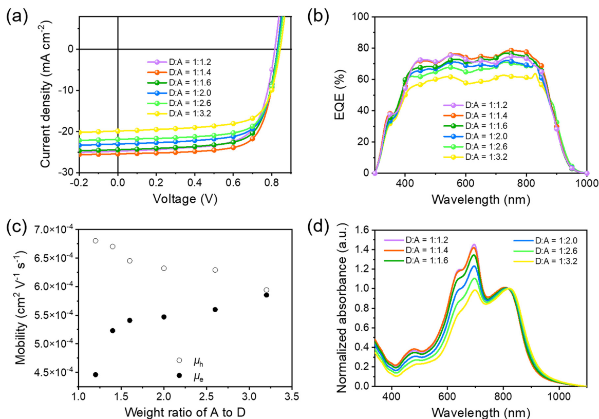
Fig. 4 (a) J–V curves of PBDTTPTP:N3 opaque solar cells with different D/A ratios. (b) EQE spectra. (c) The variation of \mu_h and \mu_e along with the A/D ratio. (d) Absorption spectra (normalized at 817 nm) of the active layer with different D/A ratios.
