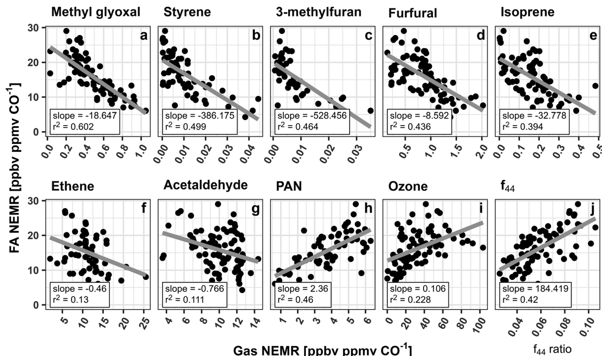
Fig. 5 FA NEMRs compared to various gas phase species NEMRs and aerosol f_{44} ratios measured in 5 smoke plumes with more than 10 pseudo-Lagrangian plume transects. Slope and r^2 for the least squares regression of each species are shown at the bottom of each panel, while the gray lines represent the best fit. Panels (a)–(c) show the three VOCs with the strongest correlation to FA. Panels (d) and (e) show two of the largest OH radical sinks (ranked by OH reactivity from individual VOC) 24 that are highly correlated with FA in wildfire emissions. Panels (f) and (g) show known FA precursors, while quantities plotted in (h)–(j) are representative of the overall plume oxidation. Note, methyl glyoxal is measured with acrylic acid ( C_3H_4O_2 ). PAN = peroxyacetyl nitrate. f_{44} = ratio of m/z 44 to the total signal in the aerosol component spectrum with higher ratios indicating more aged organic aerosol and higher O:C.
