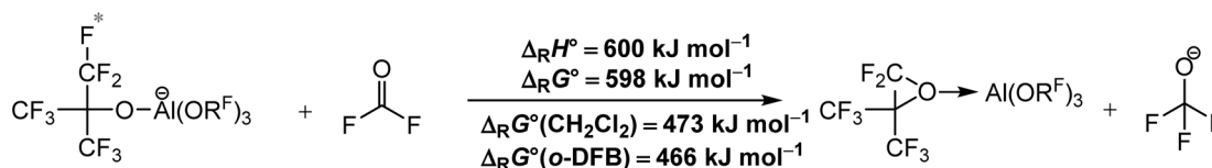
Scheme 1 Calculated isodesmic reaction enthalpies \Delta_R H^\circ and Gibbs free energies \Delta_R G^\circ for the decomposition of the [\text{Al}(\text{OR}^F)_4]^- WCAs ((1) and (2) R^F = \text{C}_{10}\text{F}_{15} ), (3) ( R^F = \text{C}(\text{CF}_3)_3 ) under fluoride ion abstraction (BP86/def-SV(P) level with D3(BJ) dispersion). Solvation effects on the Gibbs free energy \Delta_R G^\circ were considered by using the COSMO solvation model for \text{CH}_2\text{Cl}_2 ( \epsilon = 8.93^{52} ) and o -DFB ( \epsilon = 13.38^{52} ). The red star marks the abstracted fluoride ion. The experimental FIA of \text{COF}_2 of 209 \text{ kJ mol}^{-1} was used as an anchor point for comparison.
