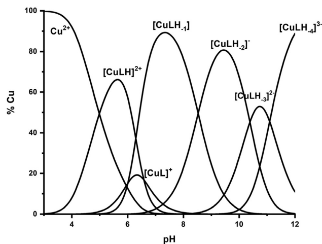
Fig. 7 Species distribution diagram of the system Cu(II)–Ac-GSTENLK \text{H-NH}_2 (R1) in a molar ratio of 1 : 1.2 ( C = 2 mM).
