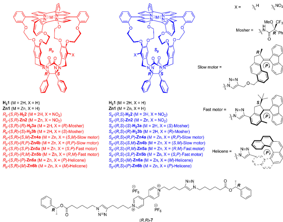
Fig. 1 Chemical structures of chiral host and guest molecules. Only the ( R )-isomer of the Mosher substituent and the ( P )-isomers of the motor and helicene substituents are shown.
