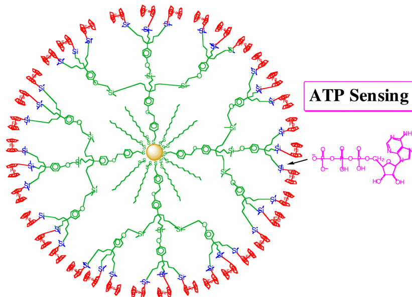
Fig. 13 ATP anion redox sensing by gold NP-centered silylferrocenyl-terminated dendrimers (planar representation). The oxygen ATP atoms interact with the electrophilic Si atoms.
