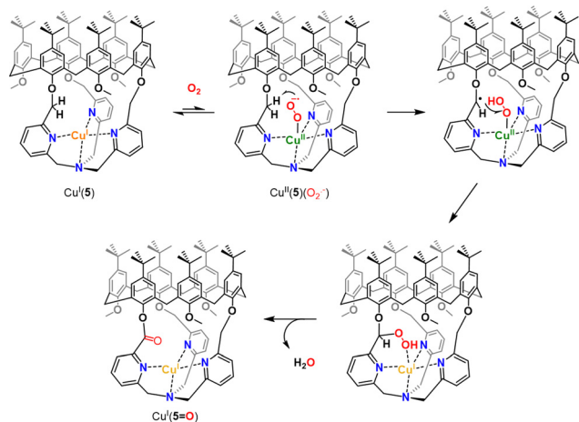
Fig. 6 Proposed mechanism for intramolecular C–H bond oxidation upon O 2 activation in Cu(5). A similar pathway is proposed for Cu(4).
