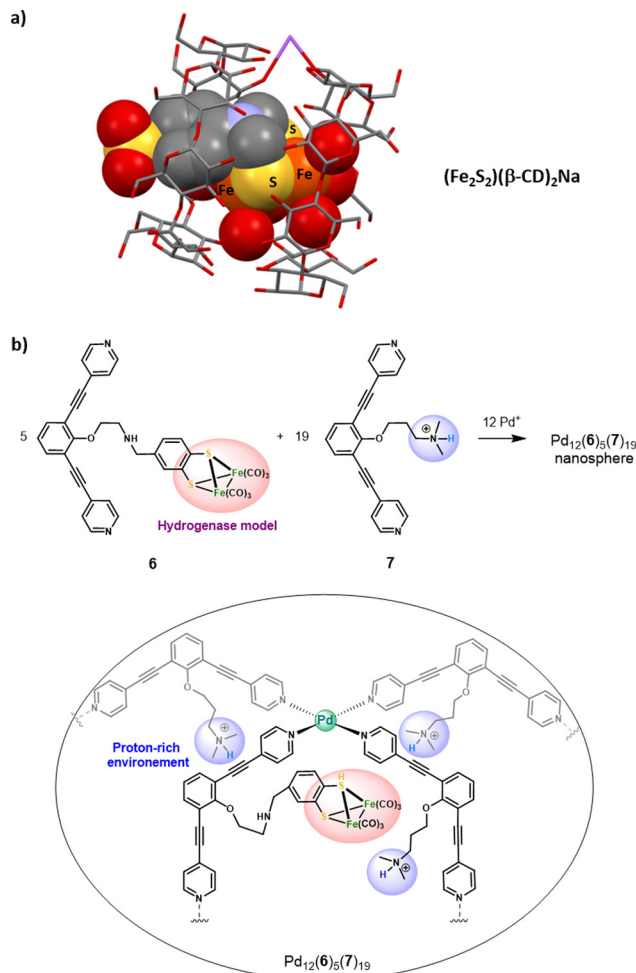
Fig. 7 (a) Representation of the XRD structure of (Fe 2 S 2 )(β-CD) 2 Na. (b) Confinement of five hydrogenase mimicking clusters in a proton rich the Pd 12 (6) 5 (7) 19 nanosphere (top), along with the schematic representation of one of the five catalytic centers found in the nanosphere (bottom).
