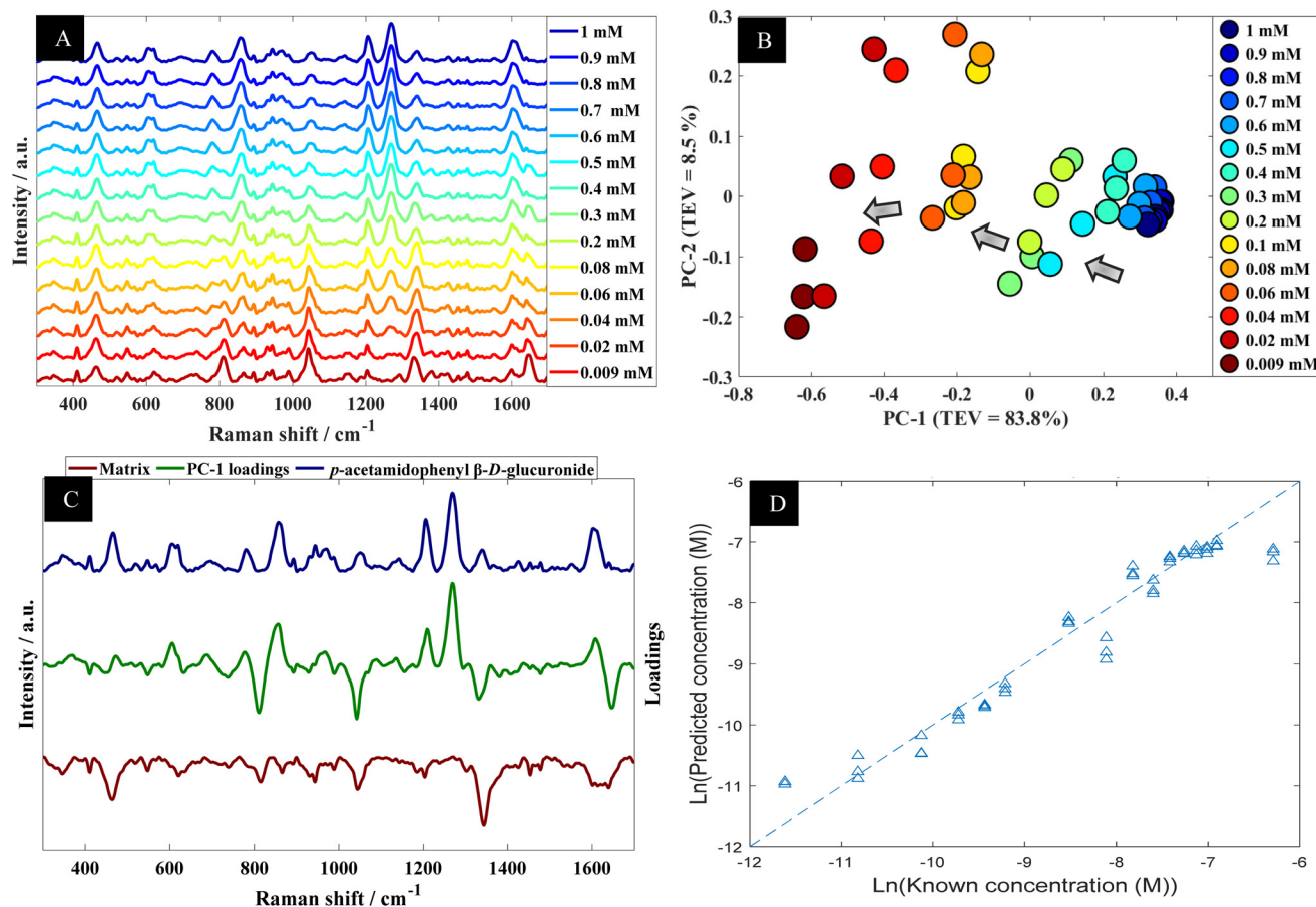
Fig. 4 (A) A series of SERS spectra of p -acetamidophenyl \beta -D-glucuronide in water at different concentration; spectra are offset for clarity. (B) PCA scores plot of SERS data acquired from p -acetamidophenyl \beta -D-glucuronide in water at different concentrations; TEV refers to total explained variance. (C) Corresponding PC-1 loadings plot (green line), with SERS spectra of p -acetamidophenyl \beta -D-glucuronide in water (blue) and matrix (brown line; this has been multiplied by (-1) for clarity). (D) PLSR quantitative output generated using SERS data from p -acetamidophenyl \beta -D-glucuronide in water; data shown are the test set outputs only from the k -fold validation procedure.
