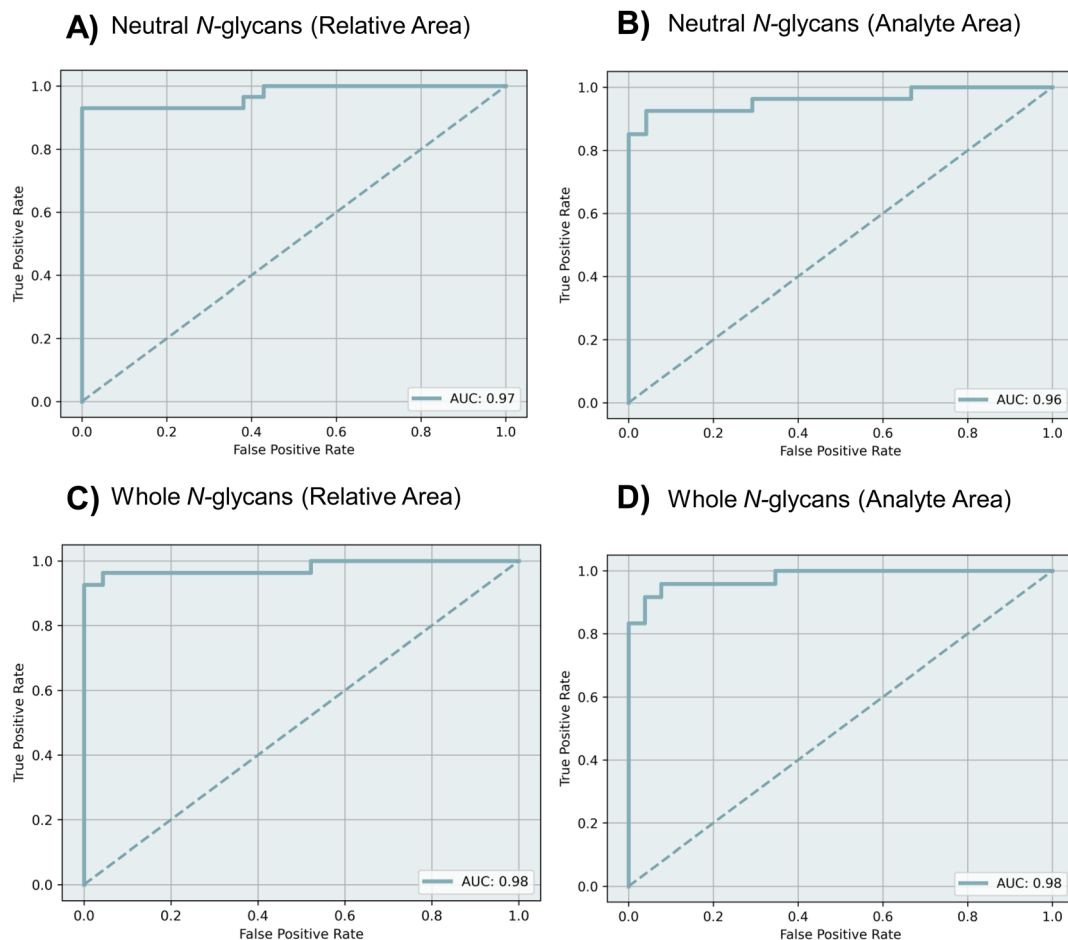
Fig. 4 ROC curves including AUC values of MLP model from different datasets (A) relative area of neutral N -glycans, (B) analyte area of neutral N -glycans, (C) relative area of whole N -glycans, and (D) analyte area of whole N -glycans.
