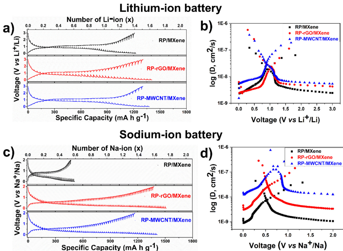
Fig. 4 GITT charge-discharge plots and corresponding \text{M}^+ chemical diffusion coefficients in the composites at various voltages: (a and b) LIB, (c and d) SIB. GITT was measured after second charge-discharge cycle to evade the effects of solid-electrolyte interface formed during first cycle.
