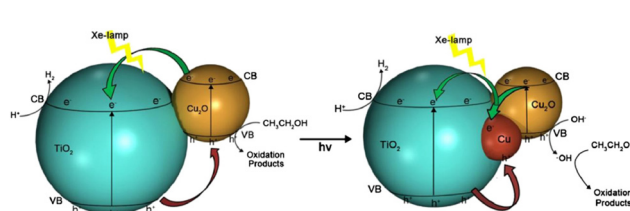
Fig. 17 H 2 -Production mechanism from photoreforming of ethanol using Cu 2 O/Cu/TiO 2 under Xe-lamp irradiation. Reprinted with permission from Elsevier. 212,214
