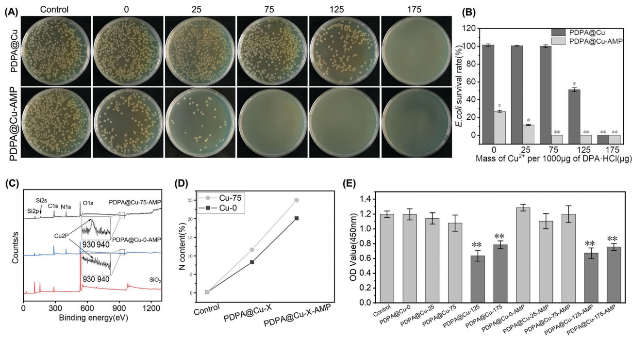
Fig. 2 (A) Bacterial growth on LB solid medium and (B) E. coli survival rate after contact with the control group, PDPA@Cu with different mass ratios of DPA to \text{Cu}^{2+} group and PDPA@Cu-AMP coating with different mass ratios of DPA to \text{Cu}^{2+} group for 24 h. (C) XPS of \text{SiO}_2 slides, PDPA@Cu-0-AMP and PDPA@Cu-75-AMP coatings. (D) Different N contents of control, PDPA@Cu-0/75, and PDPA@Cu-0/75-AMP coatings. (E) CCK8 assay of control, different rate of DPA to \text{Cu}^{2+} PDPA@Cu and PDPA@Cu-AMP coating groups. The error bars represent SD, and statistically significant differences are indicated by * p < 0.05 or ** p < 0.005 compared with the control group.
