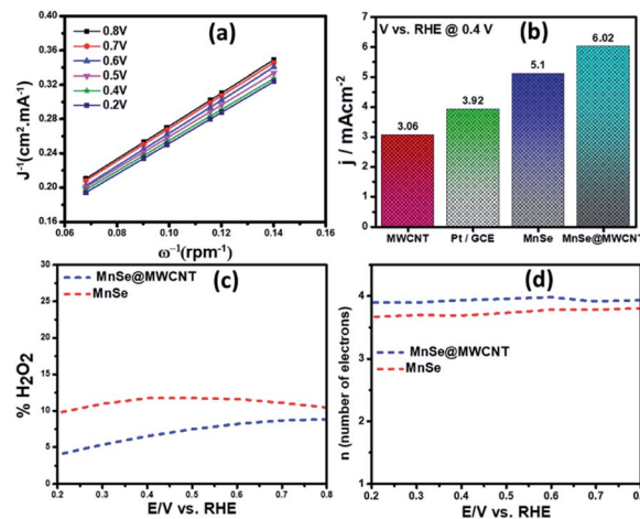
Fig. 8 (a) K–L plots of the MnSe@MWCNT composite electrode in O 2 -saturated 1 M KOH. (b) Reduction current densities of MWCNT, Pt/GCE, MnSe, and MnSe@MWCNT. (c) H 2 O 2 yield and (d) number of electrons for the MnSe@MWCNT modified electrode and MnSe at a disc rotation speed of 1200 rpm and scan rate of 10 mV s -1 in O 2 saturated 1 M KOH.
