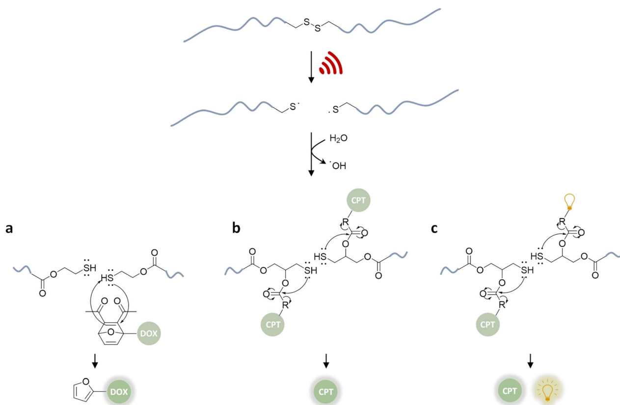
Fig. 3 US-induced scission of disulfide-centered polymers and release of drug or reporting molecules. Generated thiols undergo (a) inter-molecular Michael-addition to initiate retro Diels–Alder reaction releasing furylated doxorubicin, 79 (b) intramolecular 5- exo-trig cyclization to release camptothecin, 61 (c) intramolecular 5- exo-trig cyclization to release camptothecin and fluorescent umbelliferone simultaneously. 85
