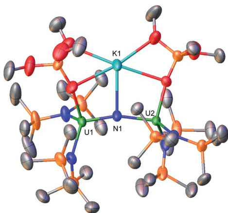
Fig. 3 Molecular structure of complex, [\text{K}\{\text{U}^{\text{III/IV}}(\text{OSi}(\text{O}^t\text{Bu})_3)_2(\mu\text{-N})\}(\mu\text{-N})][\text{K}(\text{THF})_6] , 4, with thermal ellipsoids as drawn at the 50% probability level. Hydrogen atoms, methyl groups on the \text{OSi}(\text{O}^t\text{Bu})_3 ligands, and the [\text{K}(\text{THF})_6] cation have been omitted for clarity.
