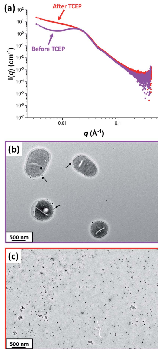
Fig. 7 (a) SAXS patterns recorded for a 1.0% w/w aqueous dispersion of PDMAC_{49} - P(HBA\text{-}stat\text{-}DAAM)_{302} vesicles (loaded with 2.5% w/w silica nanoparticles) before (purple pattern) and after TCEP addition (red pattern) confirming loss of the structure factor corresponding to the silica nanoparticles encapsulated within the vesicles. The low q gradient in the SAXS pattern recorded at 20 °C indicates the formation of worms after decrosslinking. Corresponding TEM images recorded (b) before and (c) after TCEP addition confirm the presence of silica-loaded vesicles and free silica nanoparticles, respectively. The black arrows shown in (b) indicate a few silica nanoparticles apparently adsorbed to the outer surface of the vesicles. [N.B. The linear worms formed at 20 °C in (c) cannot be observed by TEM because they undergo film formation during TEM grid preparation].
