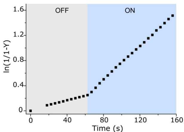
Fig. 4 Acceleration of the hydrazone reaction under constant light irradiation (blue region) after the initial \approx 60 s stay of the system (100 \mu M) in the dark (grey region), acetonitrile/ H_2O mixture ( v/v \approx 40 : 60 ), pH \approx 3 , 298 K. Note that Y stands for the product yield, and the first datapoint in the blue region corresponds to the steady state of the photoswitch.
