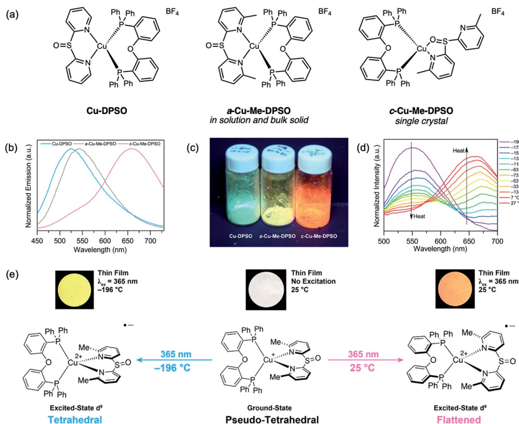
Fig. 18 (a) Structures of Cu(I) complexes Cu-DPSO and Cu-Me-DPSO reported by our group. (b) Room-temperature solid-state emission spectra of Cu-DPSO, \alpha -Cu-Me-DPSO and c -Cu-Me-DPSO (drop-cast from MeOH, \lambda_{\text{ex}} = 390 nm). (c) Photographs of the Cu(I) complexes under UV excitation. (d) Variable-temperature solid-state emission spectra of c -Cu-Me-DPSO from -196 to 27^\circ\text{C} (drop-cast from MeOH, \lambda_{\text{ex}} = 390 nm). (e) Proposed excited-state conformational changes resulting in the thermochromic emission of c -Cu-Me-DPSO. Adapted with permission from ref. 88. Copyright 2018 American Chemical Society.
