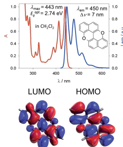
Fig. 1 Structural framework of PXX along with its fundamental optical gap properties.
