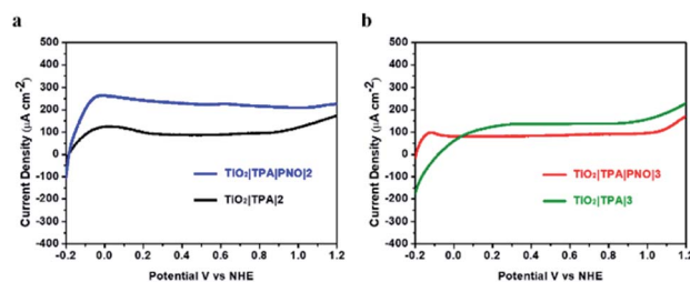
Fig. 8 Linear sweep voltammograms for (a) \text{TiO}_2|\text{TPA}|\text{PNO}|2 (blue) and \text{TiO}_2|\text{TPA}|2 , and (b) \text{TiO}_2|\text{TPA}|\text{PNO}|3 (red) and \text{TiO}_2|\text{TPA}|3 under >400 nm illumination at 100 \text{ mW cm}^{-2} in pH 7, 0.1 M phosphate buffer containing 0.4 M \text{NaClO}_4 .
