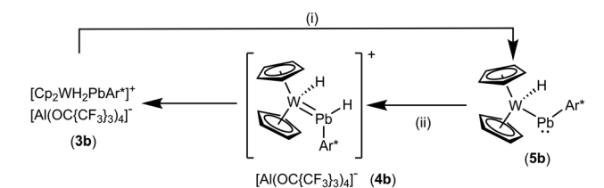
Scheme 8 (i): + Me NHC, toluene/o-DFB, rt, 3 h, – [ Me NHC–H][Al(OC{CF 3 }) 4 ], (ii): + [H(Et 2 O) 2 ][Al(OC{CF 3 }) 4 ], toluene/C 6 H 4 F 2 , rt, – 2 Et 2 O.
