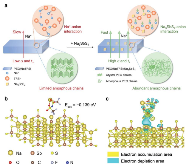
Fig. 1 Design of the interaction between the anion in salt and the additive. (a) Schematic illustrations of the PEO/NaTFSI and PEO/NaTFSI/ \text{Na}_3\text{SbS}_4 electrolytes where the interactions between \text{Na}_3\text{SbS}_4 and \text{TFSI}^- anions are highlighted by red dotted lines. (b) The optimized configuration, adsorption energy, and (c) differential charge density of NaTFSI adsorbed on \text{Na}_3\text{SbS}_4 ; the isosurface value is set to 0.0001 \text{ e Bohr}^{-3} .
