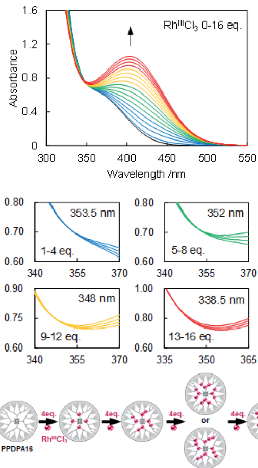
Fig. 1 Accumulation of Rh III Cl 3 to PPDA16. (top) Change in UV-vis absorption spectra of PPDA16 in DCM upon adding Rh III Cl 3 in MeCN/MeOH = 250/1 up to 16 eq. ([PPDA16] = ca. 5 \mu M, 20 ^{\circ} C). (down) Enlarged views during complexation with Rh III Cl 3 in respective positions 0–4, 5–8, 9–12, and 13–16 eq. and the schematic illustration of the possible coordination sequence.
