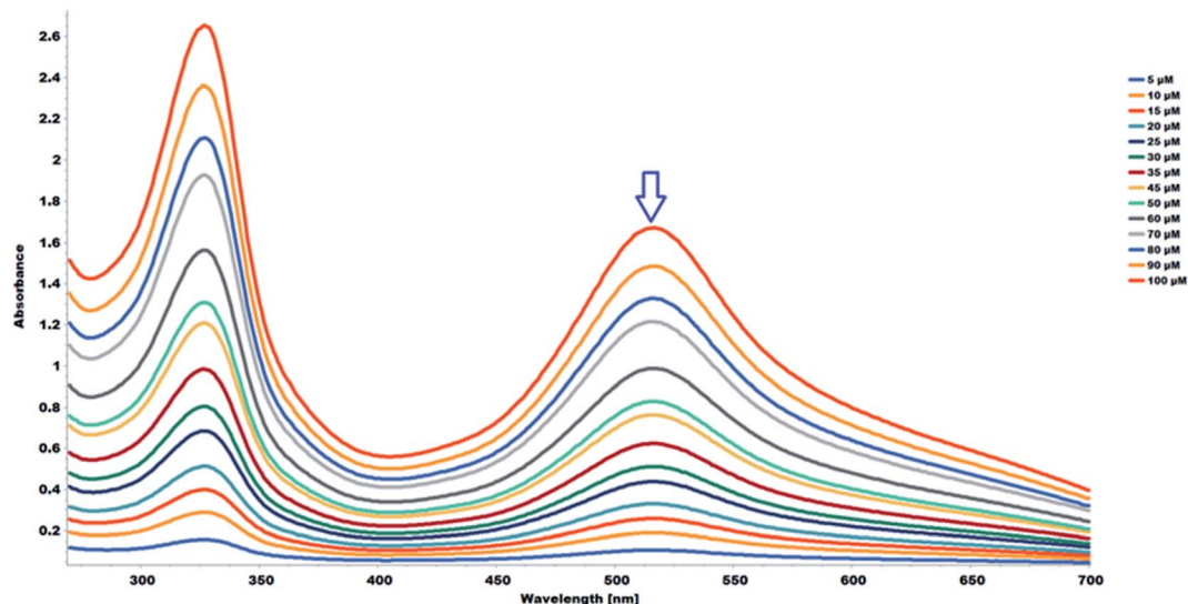
Fig. 6 UV-Vis absorption spectra (268–700 nm) in methanol of DPPH (5.0–100 \mu\text{M} ) with 100 \mu\text{L} of DMSO.
