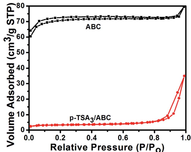
Fig. 6 N 2 adsorption-desorption isotherms of ABC and p -TSA 3 /ABC catalyst.
