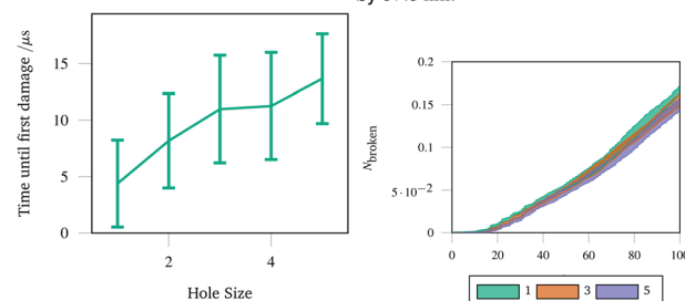
(b) Time until the first bond is broken as a function of hole size. Larger holes lead to later initial damage, as there are fewer polymers that have aged, despite system size effects. The chance to break.
