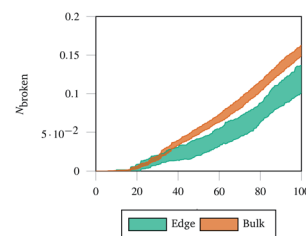
(e) Damage over time for a network with a hole of size five, tracking bonds on the edge of the hole against bonds in the bulk ("edge") against bonds away from the hole ("bulk").
