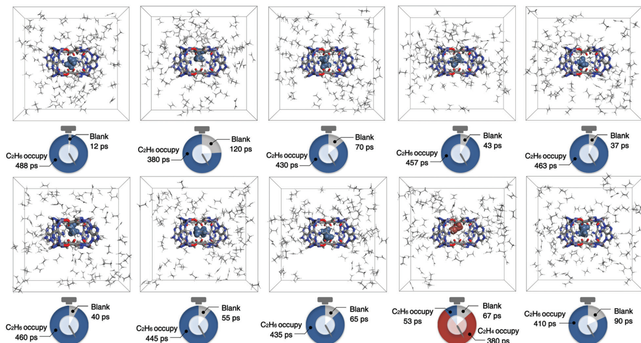
Fig. 4 Snapshots of gas molecules entering into Cage A in 10 parallel 500 ps MD simulations in a box (30 Å × 30 Å × 30 Å) filled with a C 2 H 6 /C 2 H 4 (1 : 1) mixture. The C 2 H 6 and C 2 H 4 molecules entering Cage A are coloured in lake blue and rose red respectively. The corresponding time bar represents the gas residence time in Cage A within 500 ps.
