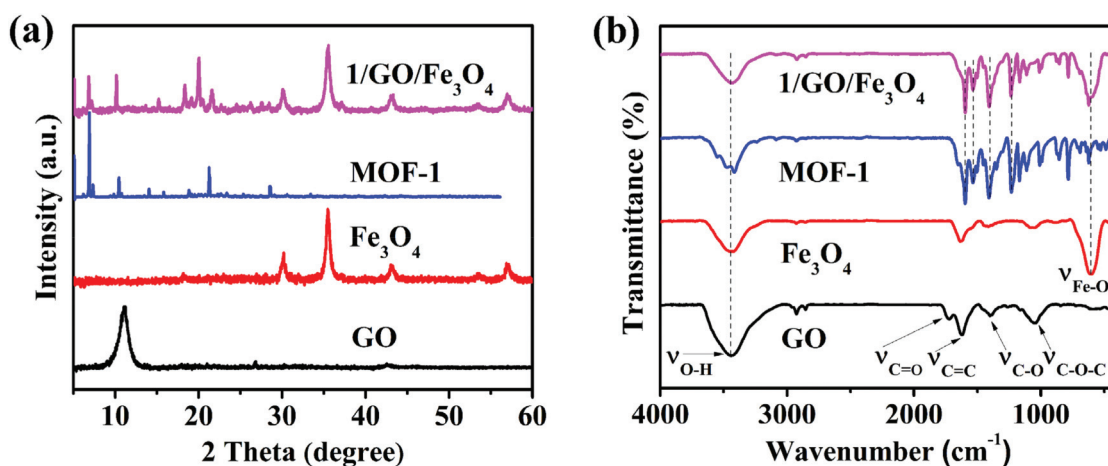
Fig. 2 PXRD patterns (a) and FT-IR spectra (b) of GO , \text{Fe}_3\text{O}_4 , MOF-1 , and 1/GO/Fe 3 O 4 (solid, temperature: 25 °C).
