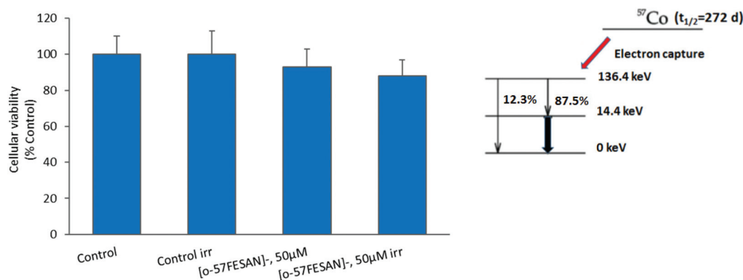
Fig. 8 Cellular viability of U87 GBM cells after irradiation with X-rays in the presence of 50 \mu\text{M} Na[o- 57 FESAN]. Irradiation was done using a Philips MCN 165 X-ray tube and a YXLON 9421 high-voltage generator at a 0.4 mGy radiation dose. ISO beam quality N120 was used ( E_{\text{max}} = 120 keV, E_{\text{ave}} = 100 keV, filtered with 4 mm Al + 5 mm Cu + 1 mm Sn).
