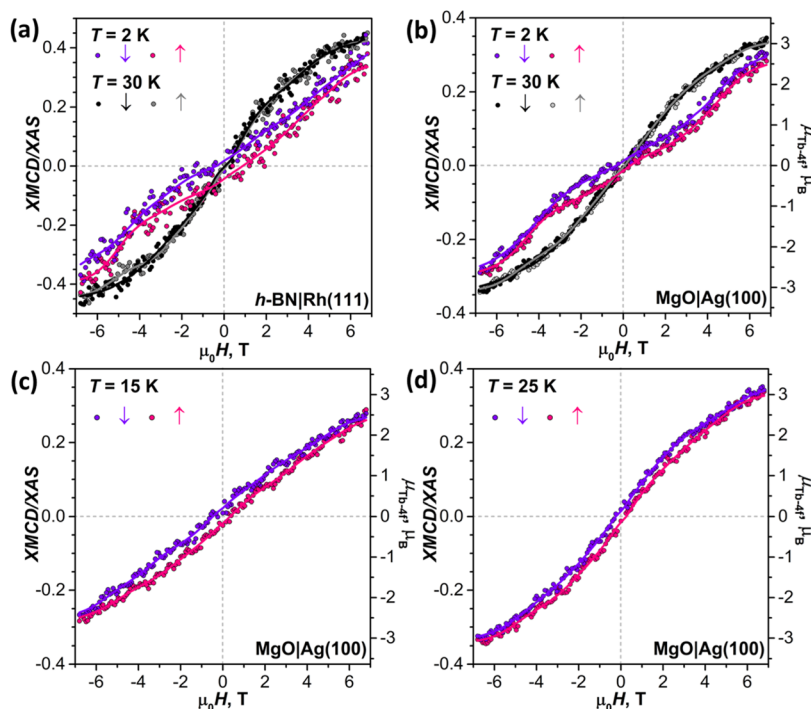
Fig. 9 (a) Magnetization curves of a Tb_2@C_{79}N submonolayer on h\text{-BN|Rh(111)} at 2 K and 30 K. (b) Magnetization curves of Tb_2@C_{79}N 1.5 ML on \text{MgO|Ag(100)} at 2 K and 30 K. (c and d) Magnetic hysteresis of Tb_2@C_{79}N 1.5 ML on \text{MgO|Ag(100)} measured at 15 K (c) and 25 K (d). All curves are measured in grazing incidence ( 30^\circ ); magnetic field sweep rate is 1.5\text{ T min}^{-1} ; dots are experimental measurements, lines are smoothed experimental data and are shown to guide the eye only; arrows denote the measurements during decrease ( \downarrow ) and increase ( \uparrow ) of the magnetic field; Tb-4f magnetic moment scale ( \mu_{Tb-4f} ) is obtained from a sum rule analysis.
