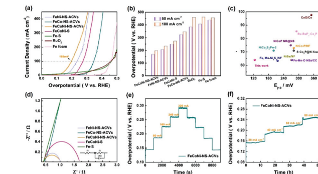
Fig. 3 Electrochemical measurements: (a) OER polarization curves, (b) overpotential comparison at 50\text{ mA cm}^{-2} and 100\text{ mA cm}^{-2} , (c) comparison of the overpotentials ( E_{j10} ) and Tafel slopes with the references, (d) Nyquist plots, and (e and f) stability tests of the obtained catalysts in 1 M KOH.
