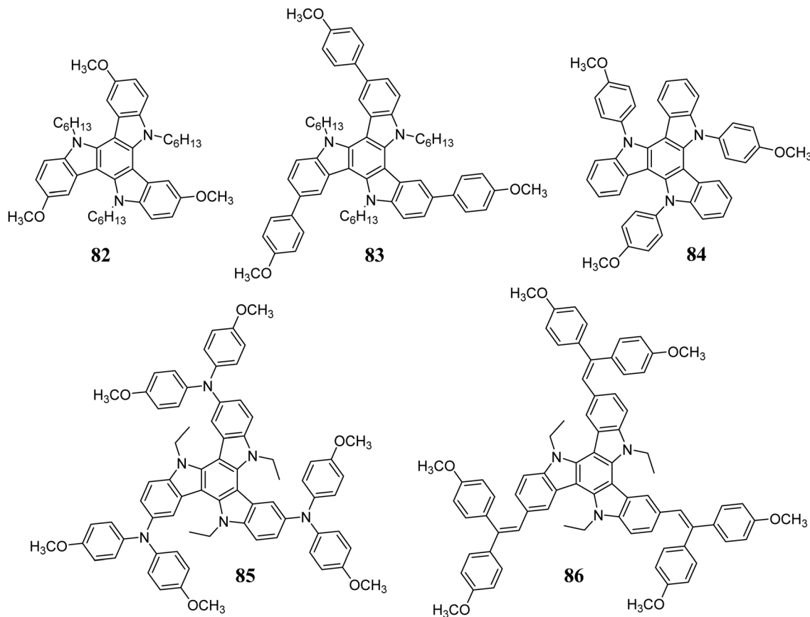
Scheme 29 5,10,15-Triazatruxene-based HTMs.
