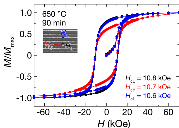
Fig. 4 Magnetic hysteresis loops ( M-H curves) of (\text{Co/Pt})_6 nanowires on \text{Si/SiO}_2 substrates after annealing at 650^\circ\text{C} for 90 min. M-H curves were measured in a vacuum at room temperature ( 27^\circ\text{C} ) by applying a magnetic field in the out-of-plane direction (perpendicular; black curves and filled circles), in-plane direction parallel to the nanowire-axis (longitudinal; red curves and filled circles), and in-plane direction perpendicular to the nanowire-axis (transversal; blue curves and filled circles). H_{c\perp} , H_{c\parallel} , and H_{c\text{b}} represent H_c for perpendicular, longitudinal, and transversal directions, respectively.
