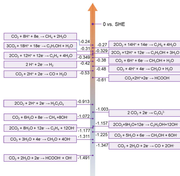
Fig. 7 \text{CO}_2 RR at different standard potentials in aqueous solution at pH = 7.0, 1.0 atm, and 25°C. Reprinted with permission from ref. 26, copyright© 2019 The Royal Society of Chemistry.
