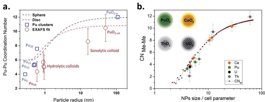
Fig. 17 (a) Comparison of the size dependence of the Pu–Pu coordination sphere when comparing EXAFS experimental data with calculations from geometrical models for \text{PuO}_2 nanoparticles. In the figure, red circles represent the experimental data: SAXS vs. EXAFS fit, whereas the blue squares result from theoretical calculations in agreement with the published crystallographic structures. Reproduced from Mischeau et al. 94 with permission from the Royal Society of Chemistry, copyright 2020. (b) Similar approach using a structural model described by the equation eqn (15) for \text{PuO}_2 and \text{CeO}_2 samples. Reproduced from ref. 201 with permission from the International Union of Crystallography, copyright 2022.
