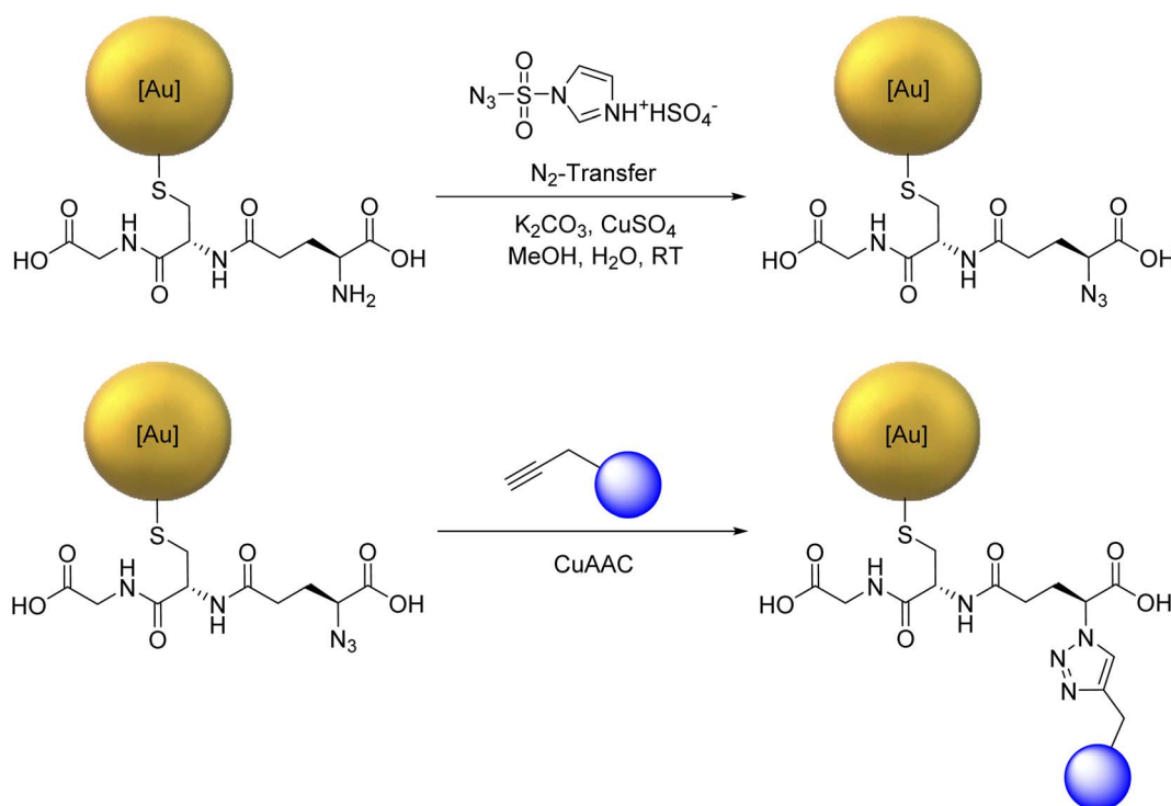
Fig. 1 Reaction scheme for the attachment of alkyne-terminated siRNA (depicted as blue balls).
