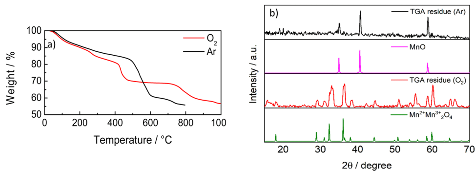
Fig. 6 (a) TGA curves of C-50 in Ar and O 2 at 10 °C min -1 . (b) XRD patterns of the residues from the TGA of Fig. 6a, MnO (reference code 01-075-0626) and Mn 3 O 4 (reference code 01-089-4837).
