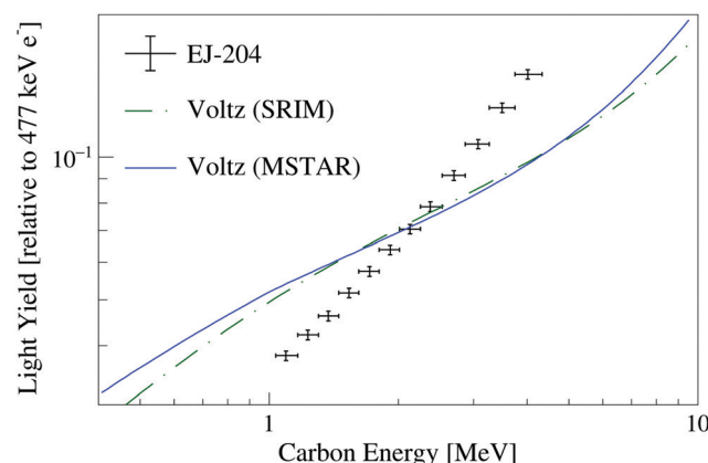
Fig. 8 EJ-204 carbon light yield data along with Voltz et al. models obtained via a simultaneous fit of EJ-204 proton and carbon light yield using the SRIM and PSTAR/MSTAR stopping power tables.
