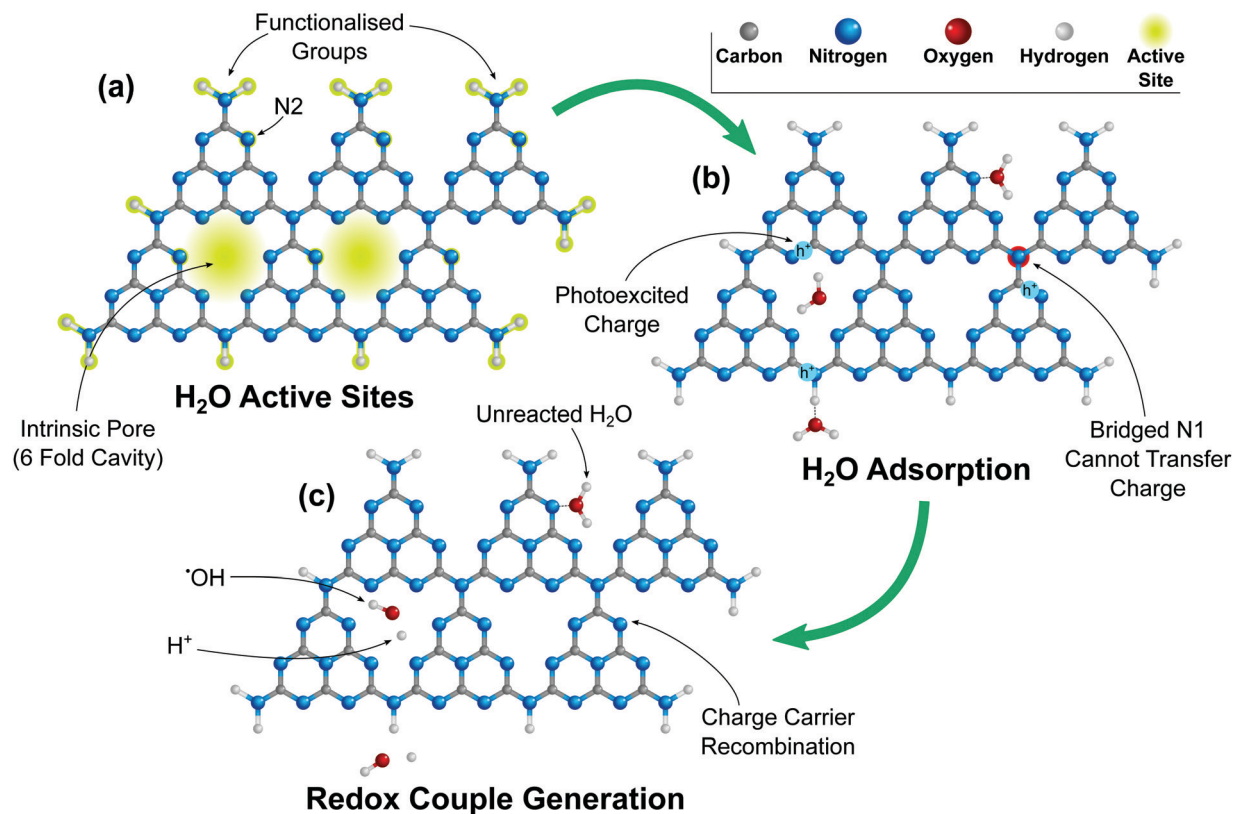
Fig. 8 Schematic diagram of g\text{-C}_3\text{N}_4 (tri-s-triazine (heptazine)) showing (a) \text{H}_2\text{O} adsorption sites, highlighted in yellow (b) \text{H}_2\text{O} adsorption onto g\text{-C}_3\text{N}_4 active sites, and electron trapping due to the bridged N1 preventing electron transfer between structural elements. 145 (c) Subsequent dissociation of \text{H}_2\text{O} into \cdot\text{OH}/\text{O}^+ redox couple where sufficient charge carriers are available.
