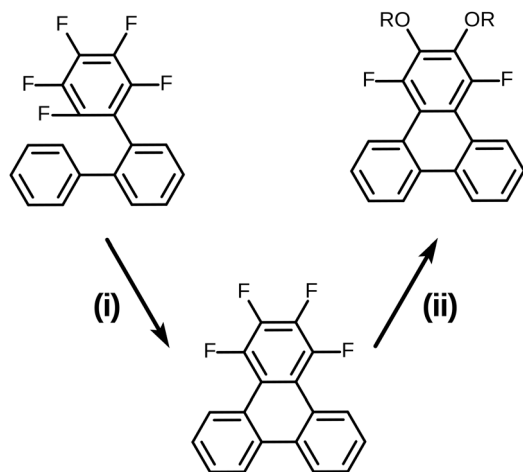
Scheme 3 Synthesis of the model S_NAr substrate and its use in the double S_NAr reaction. (i) PCDHF/acetonitrile 94%; (ii) t\text{-BuOK} (8 eq.) in excess R-OH/toluene.
