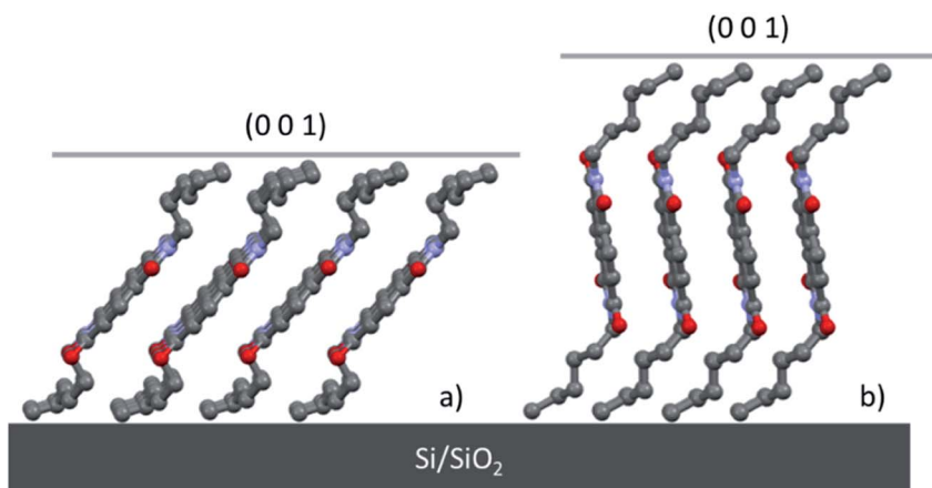
Fig. 9 Molecular arrangement of thin films oriented in the \text{Si/SiO}_2 substrates of (a) Form \alpha and (b) Form \gamma .
