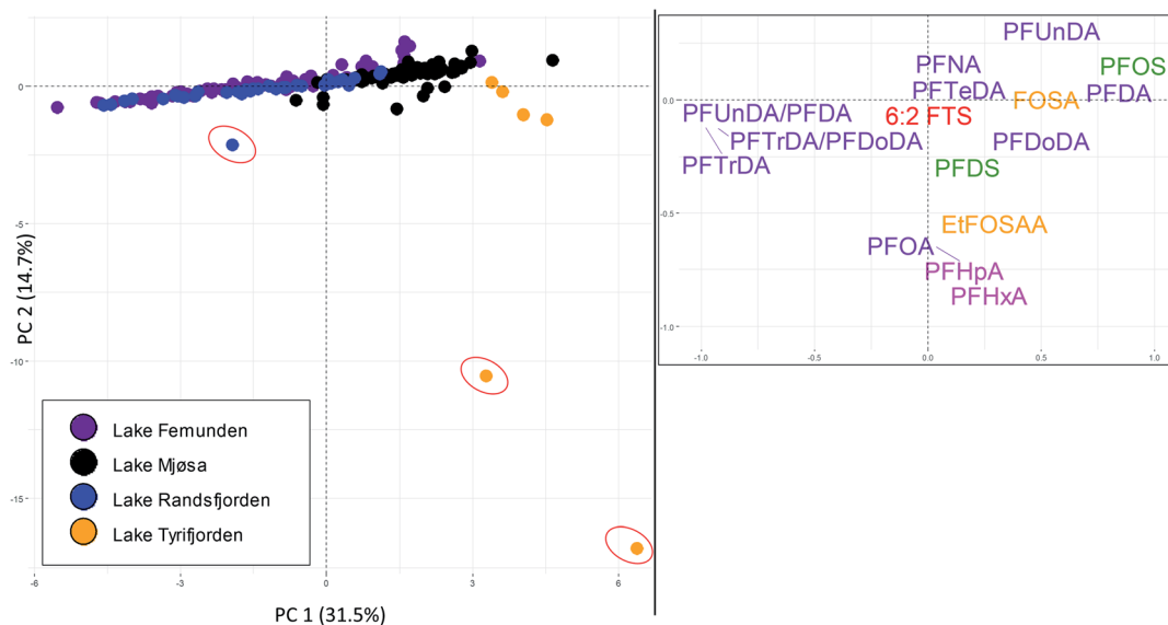
Fig. 4 Principal Component Analysis (PCA) for PFAS profiles (relative distribution profiles) in brown trout livers from four large Norwegian lakes: lake Femunden, lake Mjøsa, lake Randsfjorden, and lake Tyrifjorden. The score plot is shown to the left and the loading plot is shown to the right. Only PFAS targeted at all sites and detected above the LOQ in at least one sample were included. Concentrations below the LOQ were treated as 0. Red circles in the score plot indicate the three individuals with PFOA concentrations above the LOQ.
