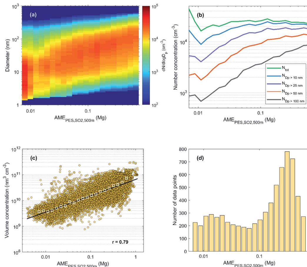
Fig. 11 (a) Hourly median particle number size distribution, (b) number concentrations and (c) total volume concentration as a function of \text{AME}_{\text{PES},\text{SO}_2,500\text{m}} during 2018–2019 in Beijing. Panel (d) shows the number of data points (hourly median values) in each bin of (a) and (b). For the calculation of the total aerosol volume in panel (c) DMPS data was used instead of the PSD data used in (a) and (b) due to more continuous data coverage and negligible contribution of the smallest (sub 6 nm) particles. In panel (c) the colored circles represent hourly median data and the white squares show the bin median values. The fit and the Pearson's correlation coefficient ( r ) in panel (c) correspond to the hourly (non-binned) data.
