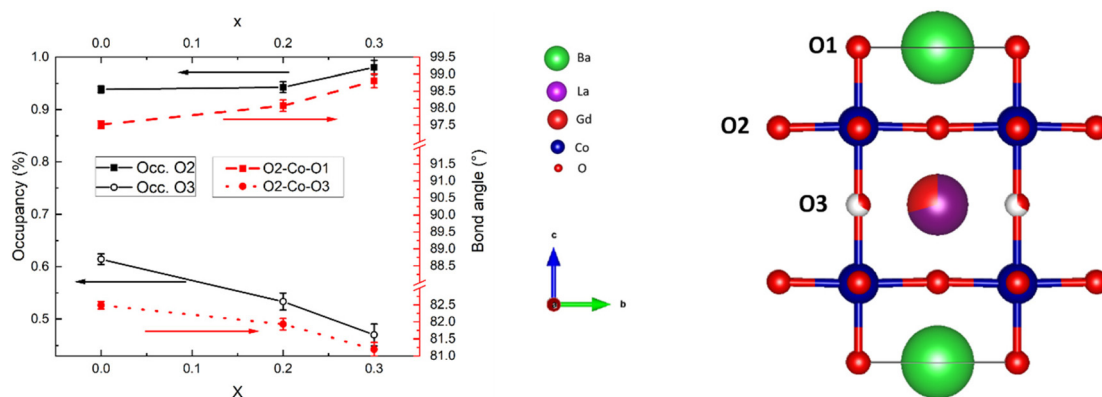
Fig. 7 SR-PXD data at room temperature showing occupancies on O2 and O3 sites (left axis) and shift in O2-Co-O1 and O2-Co-O3 bond angles (right axis) with increasing La substitution x .
