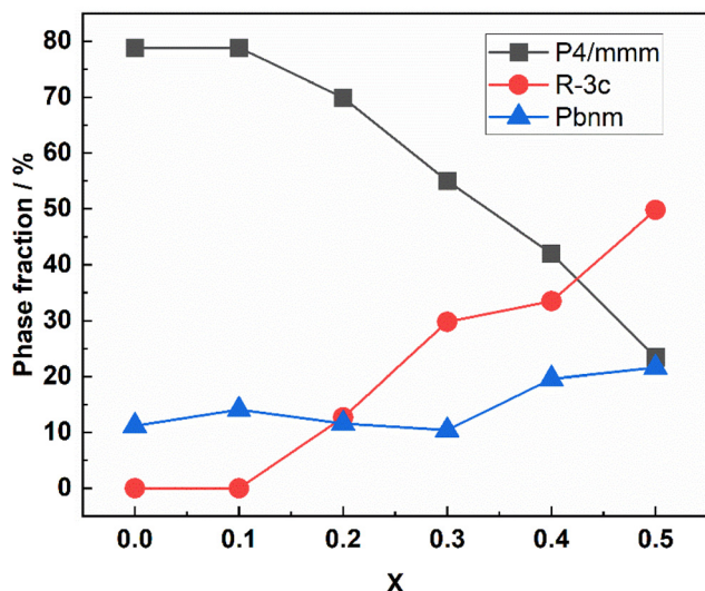
Fig. 3 Phase fractions (wt%) vs. x in BGLC ( y = 0.2 ).
