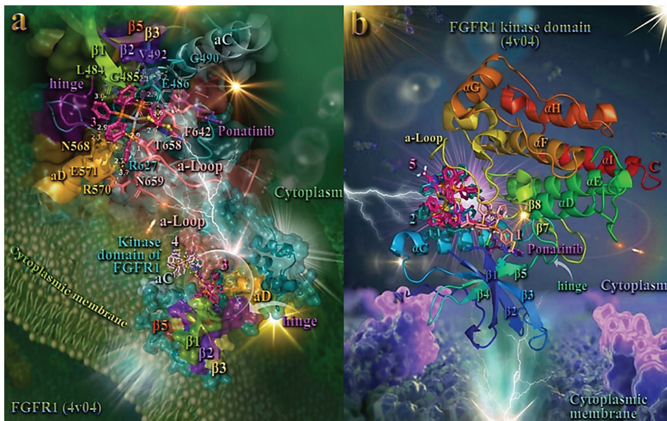
Fig. 7 (a) (lower panel) Docking pose orientation of 4 (best bound complex in in silico studies) and 3 (exhibiting the highest in vitro anticancer activity), in the crystal structure of the catalytic domain of fibroblast growth factor receptor 1 (FGFR1) kinase in complex with its inhibitor drug ponatinib (PDB accession number: 4V04). FGFR1 is localized in the cytoplasmic membrane towards the intracellular cytoplasm (transmembrane and extracellular domains are not shown). (upper panel) A close-up view of the ATP-binding site architecture of the second-best binding complex 3 . Target protein in both structure models is illustrated as cartoon colored in deep teal with depth cue in the ray-tracing rendering of the whole structure, with additional depiction of semi-transparent surface colored according to cartoon. Docked complexes 3 and 4 , as well as the superimposed co-crystallized inhibitor ponatinib, all rendered in ball-and-stick mode and colored according to atom type in warm pink, light pink, and violet purple, respectively. Selected contacting amino acid residues of the binding pocket are rendered in stick model and colored according to protein's segments: activation loop (a-Loop) (deep salmon), aC and aD helices (pale cyan and bright orange, respectively), \beta 1 , \beta 2 , \beta 3 , and \beta 5 antiparallel beta sheets (split pea green, purple blue, yellow-orange, and firebrick red, respectively), and hinge (deep purple), highlighting also the mapped surface of the corresponding part of the interacting residues in the same colors. A-loop is depicted in its active (open) conformation. Complex 3 is found to be anchored in the vicinity of the ATP-binding cleft, at the same place with ponatinib. (b) Docking pose orientation of 1 , 2 , and 5 in the crystal structure of the catalytic domain of fibroblast growth factor receptor 1 (FGFR1) kinase in complex with its inhibitor drug ponatinib (PDB accession number: 4V04). FGFR1 is localized in the cytoplasmic membrane towards the intracellular cytoplasm (transmembrane and extracellular domains are not shown). Target protein is illustrated as cartoon colored in rainbow. Docked complexes 1 , 2 , and 5 , as well as the superimposed co-crystallized inhibitor ponatinib, all rendered in stick mode and colored according to atom type in salmon, teal, hot pink, and violet purple, respectively. FGFR1 protein's segments: activation loop (a-Loop), aC and aD helices, \beta 1 , \beta 2 , \beta 3 , and \beta 5 antiparallel beta sheets, and hinge, are depicted in the structure colored according to cartoon. A-loop is depicted in its active (open) conformation. Complex 1 is found adjacent to ponatinib at the ATP-binding cleft of the protein. Molecular docking simulations of all molecules were performed individually. Binding contacts are shown as dotted yellow lines. Heteroatom color-code: O: red, N: blue, S: yellow, P: orange, F of ponatinib: cyan, F: cyan, and Ag: grey. Hydrogen atoms are omitted from all molecules for clarity. The final structure was ray-traced and illustrated with the aid of PyMol Molecular Graphics Systems. Binding interactions are shown in Table S15.†
