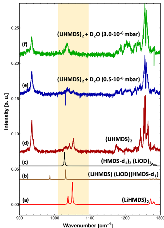
Fig. 3 Infrared spectra of \text{LiHMDS} - \text{D}_2\text{O} complexes. (a) Calculated IR spectrum of (\text{LiHMDS})_2 (B3LYP-D3/def2-TZVP, scaled by 0.992). (b) Calculated IR spectrum of (\text{LiHMDS})(\text{LiOH})(\text{HMDS}-d) (B3LYP-D3/def2-TZVP, scaled by 0.992). (c) Calculated IR spectrum of (\text{HMDS}-d_1)(\text{LiOD})_2 (B3LYP-D3/def2-TZVP, scaled by 0.992). (d) IR spectrum of (\text{LiHMDS})_2 . (e) IR spectrum of (\text{LiHMDS})_2 + \text{D}_2\text{O} with a partial pressure of 0.5 \times 10^{-6} mbar. (f) IR spectrum of (\text{LiHMDS})_2 + \text{D}_2\text{O} with a partial pressure of 3.0 \times 10^{-6} mbar.
