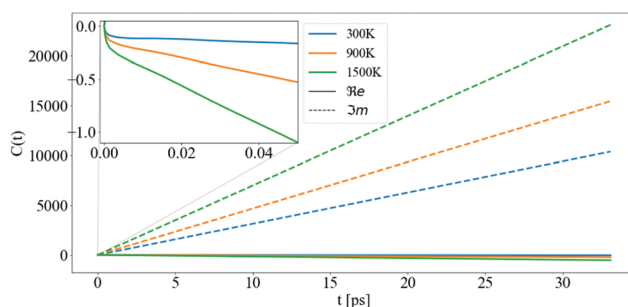
Fig. 7 The cumulant function for CBM between 0 and 32 ps, for different temperatures: 300, 900 , and 1500 K. The solid and the dashed lines are the real and imaginary parts of the cumulant function, respectively. The inset shows the non-linear behaviour of \Re e C(t) at small t .
